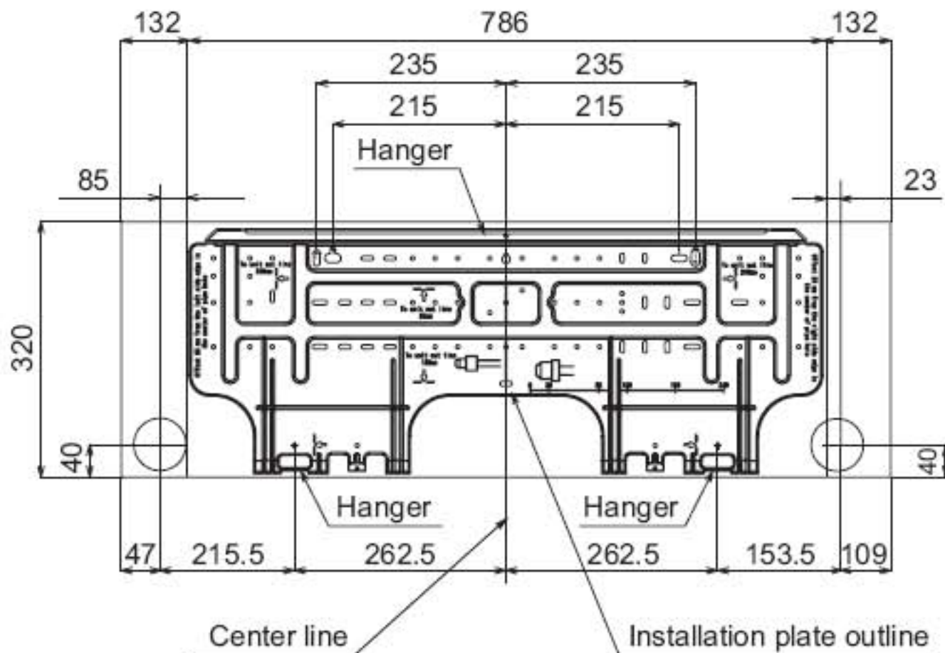
Installation plate
